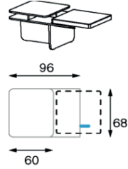
FL 006 end element with double-deck table top
