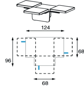
FL 011 t-element with table top
