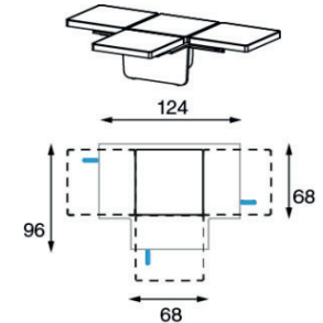
FL 012 t-element with 1 seat cushion
